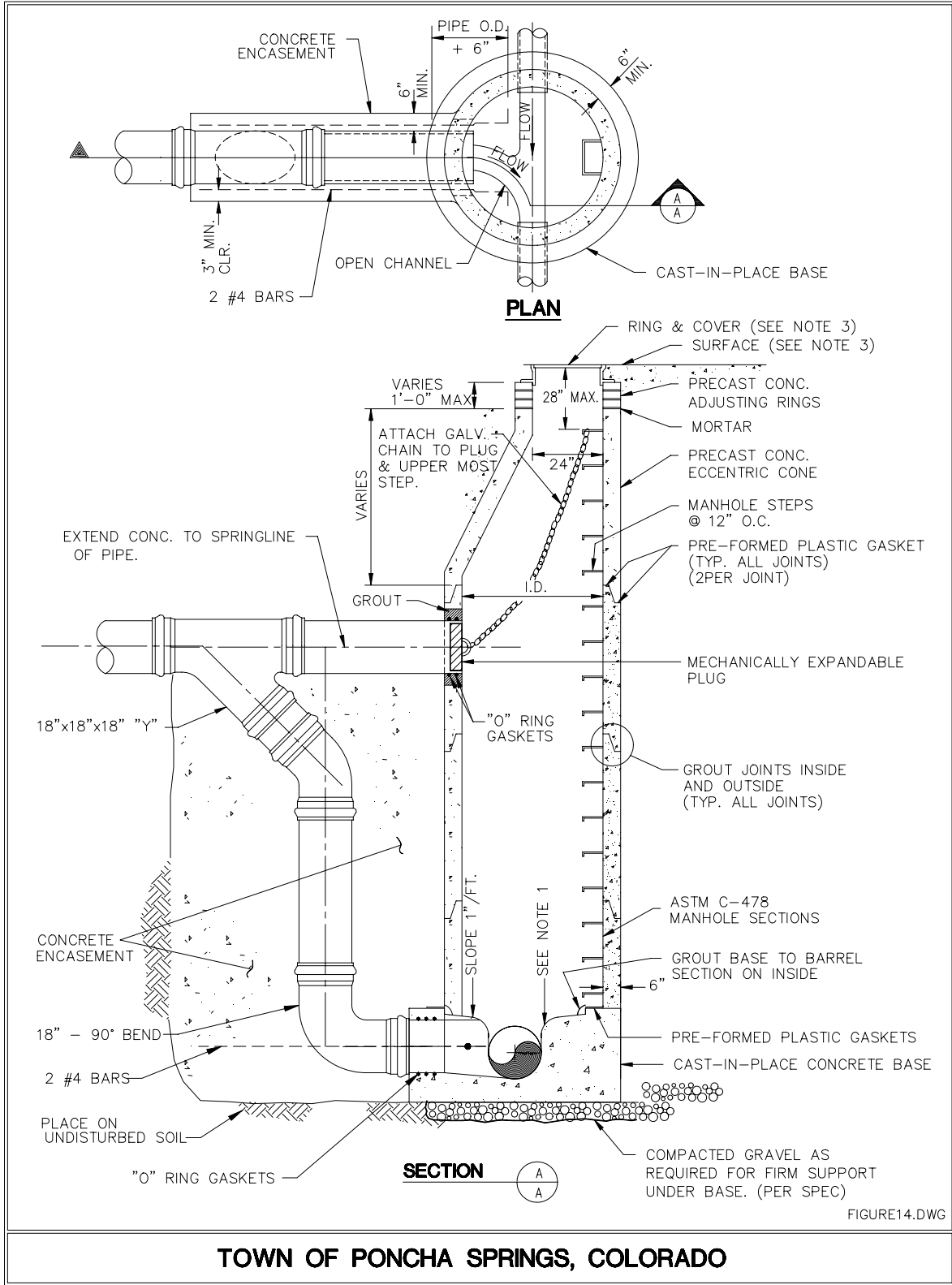
FIGURE 14 DROP MANHOLE DETAIL
