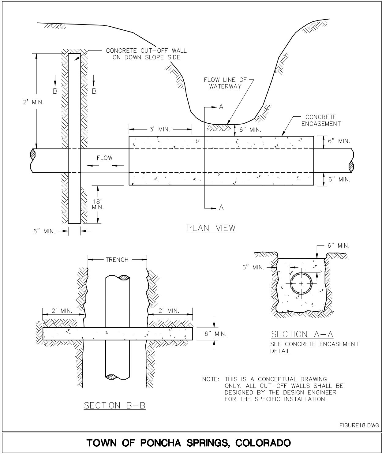
FIGURE 18 DITCH CROSSING DETAIL
