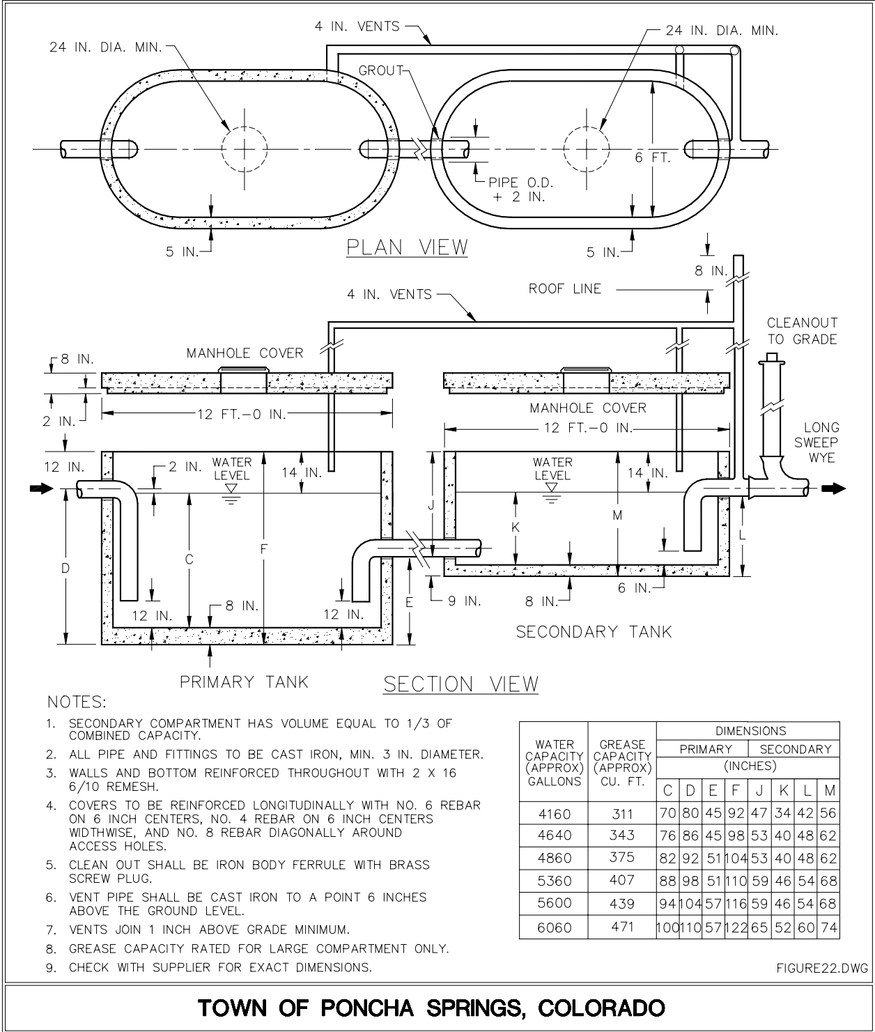
FIGURE 22 TYPE C GREASE INTERCEPTOR
