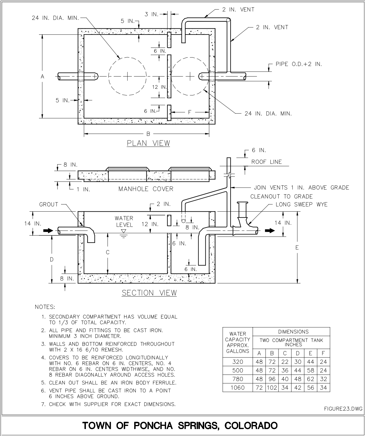
FIGURE 23 TYPE A SAND AND OIL INTERCEPTOR
